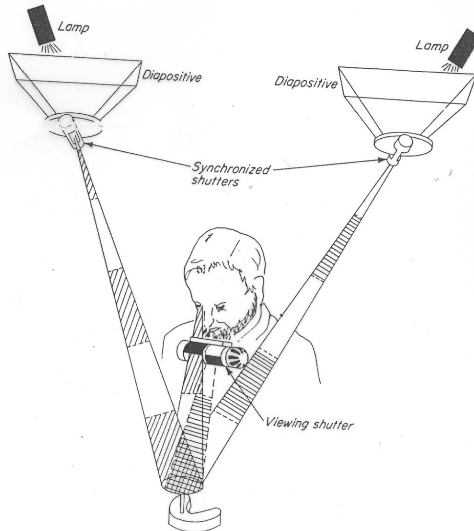
Figure 5-20. Principle of stereo image alternator (SIA).
